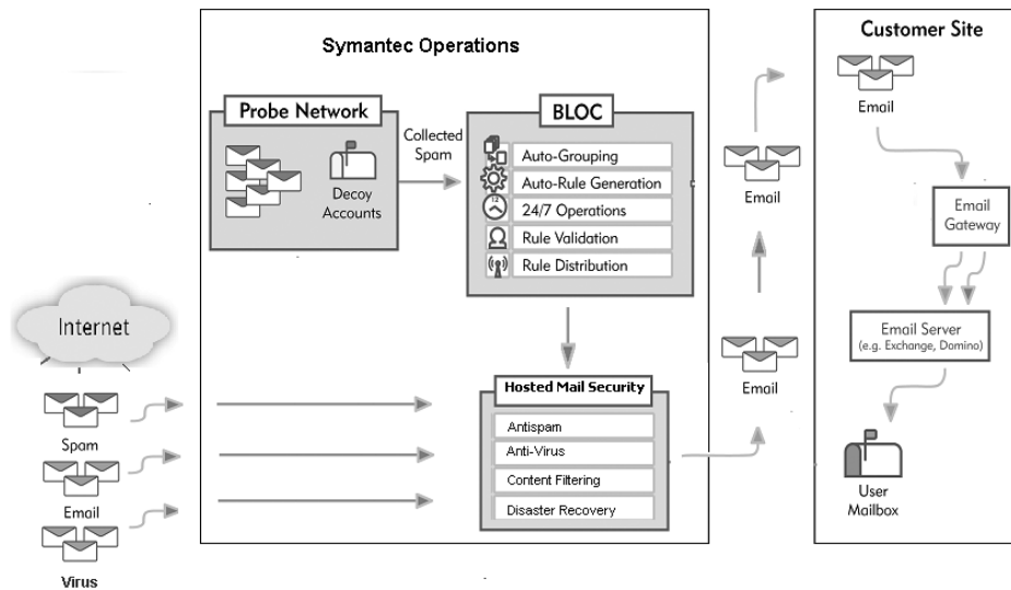
Symantec Hosted Mail Security Architecture
